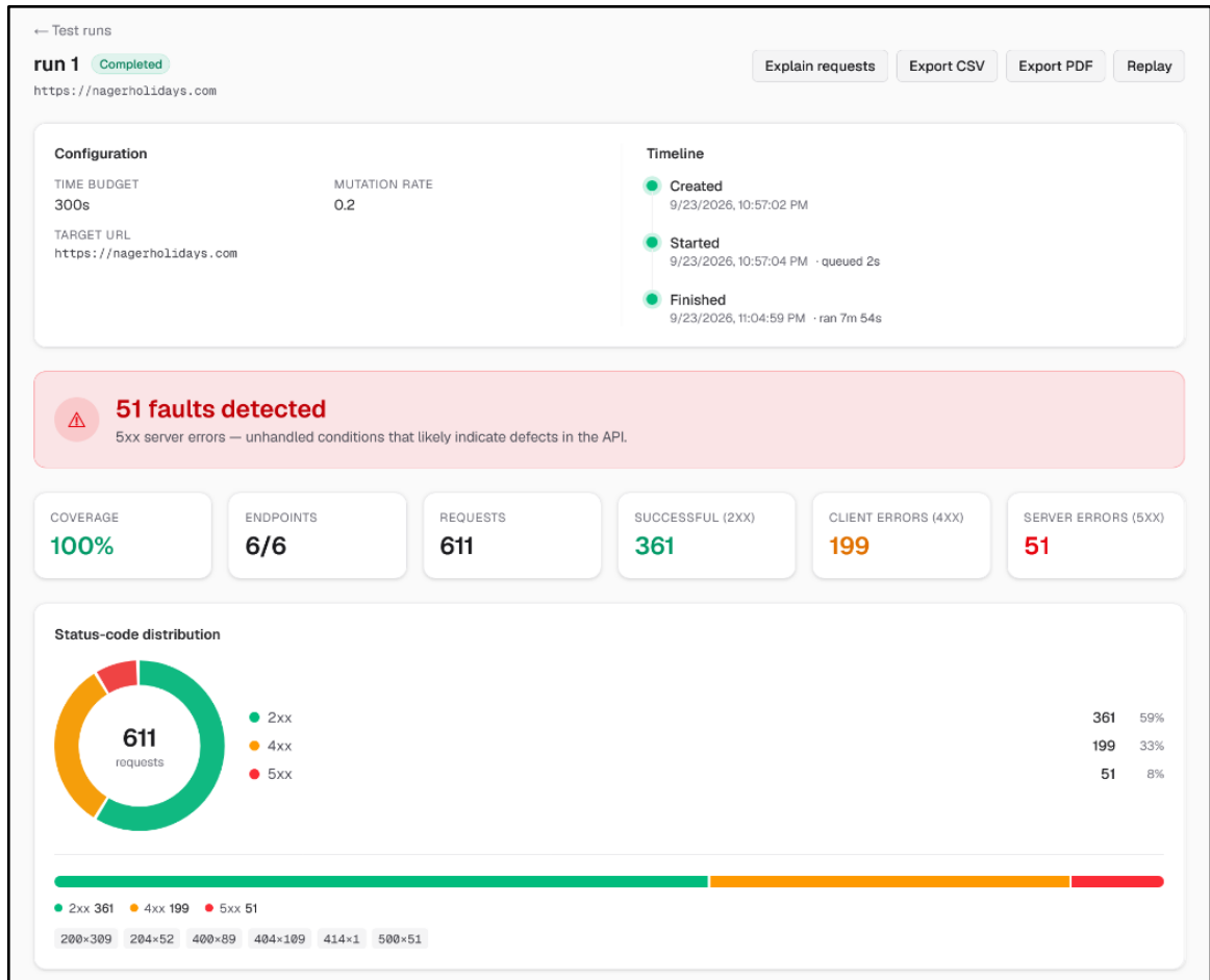
Figure 32: Test report
