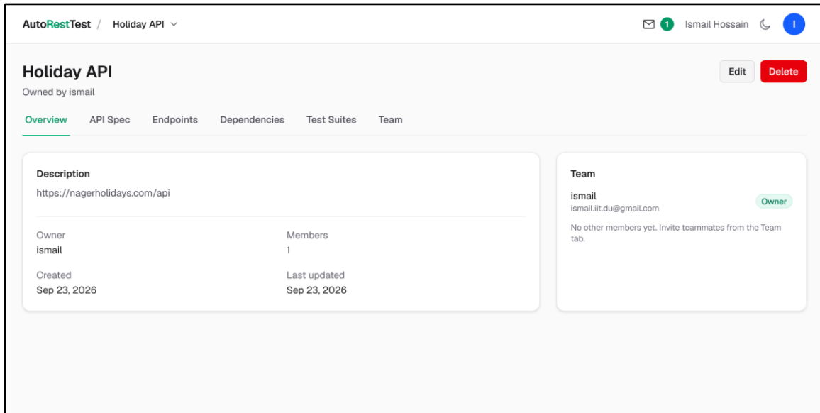
Figure 27: Project overview
