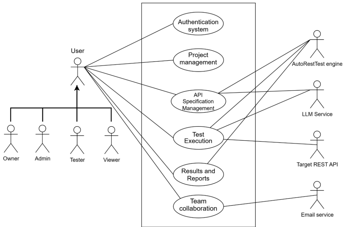
Figure 2: Use case diagram — Level 1: AutoRestTest Full system
