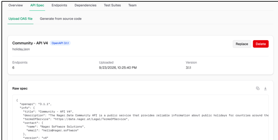
Figure 28: API Specification management
