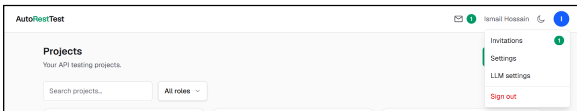
Figure 24: Navbar
