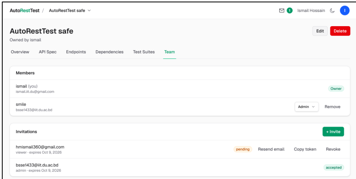
Figure 33: Team collaboration management
