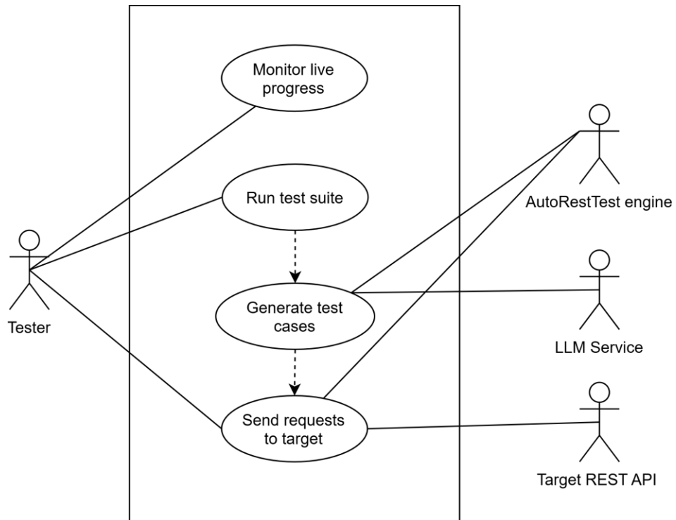
Figure 7: Use case diagram — Level 1.5: Test Execution
