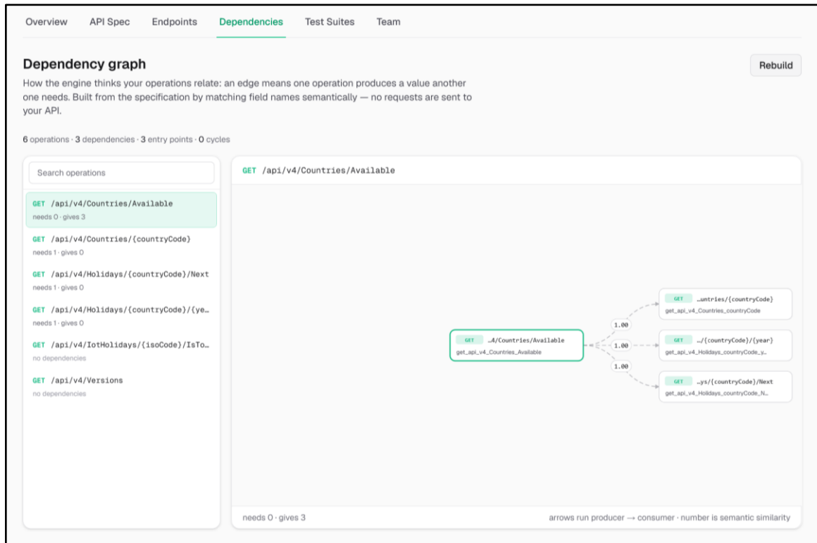
Figure 32: SPDG Visualization
